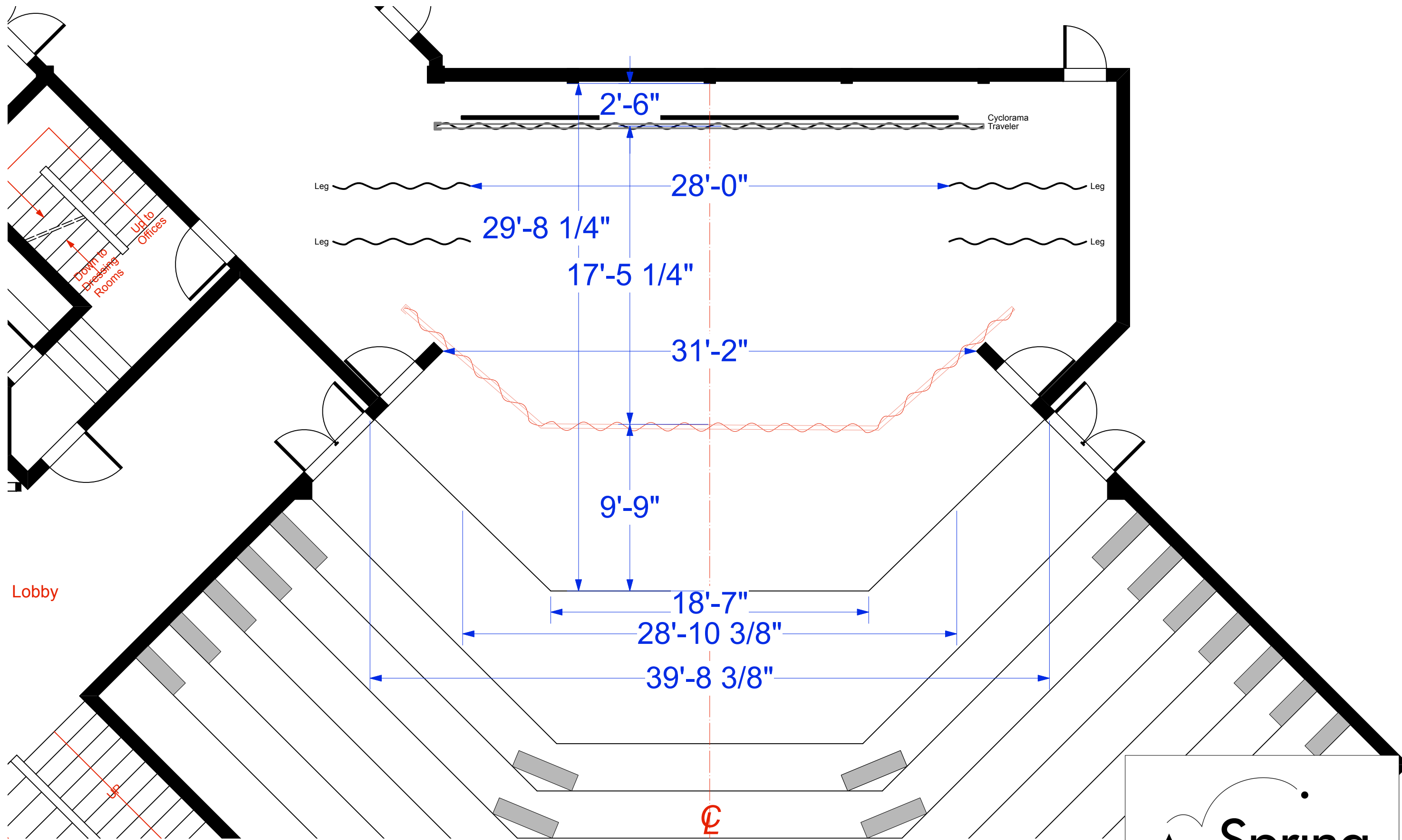
1 Stage Dimensions Scale: 3/16" = 1'-0"
