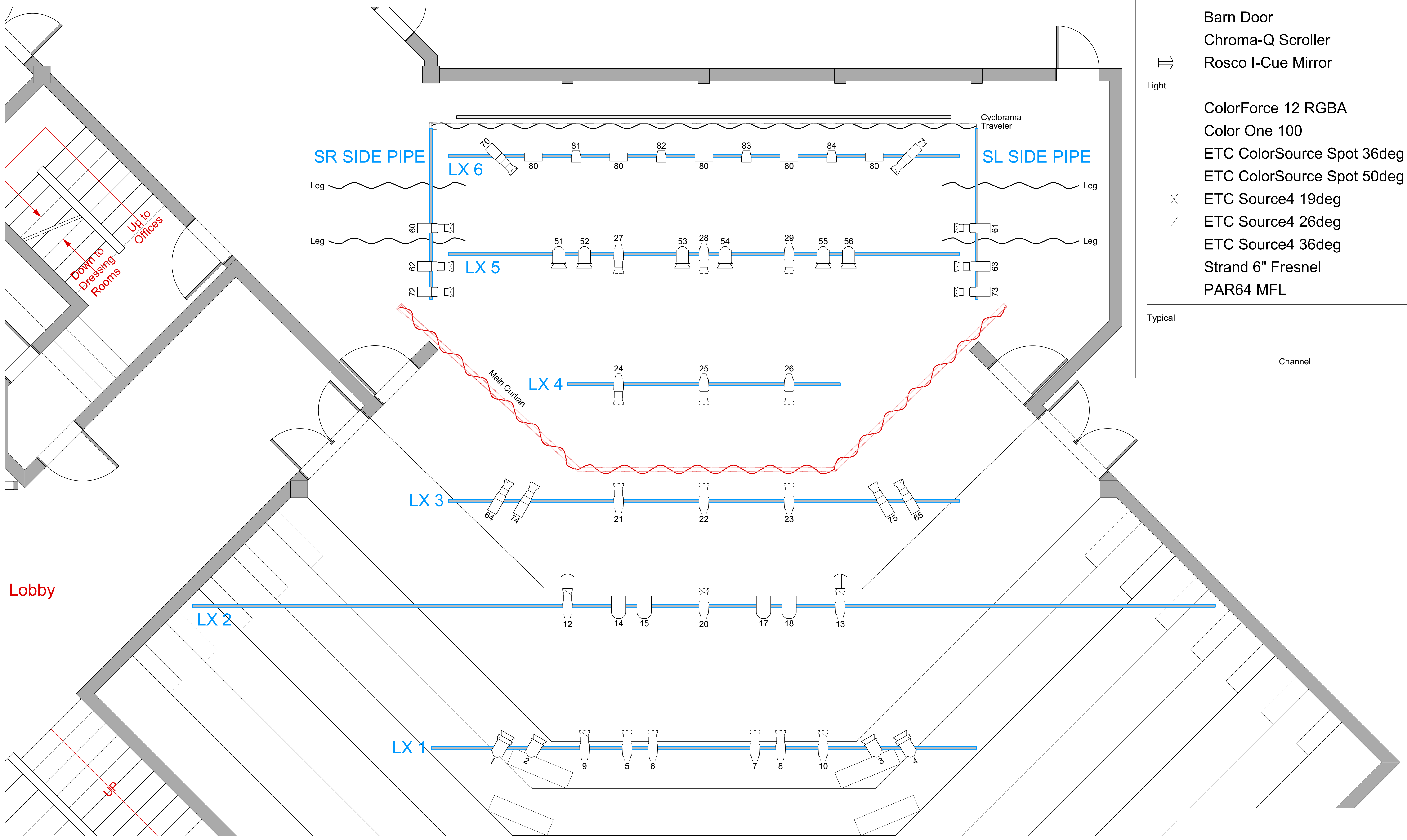
1 Lighting Plot Scale: 3/8" = 1'-0"
